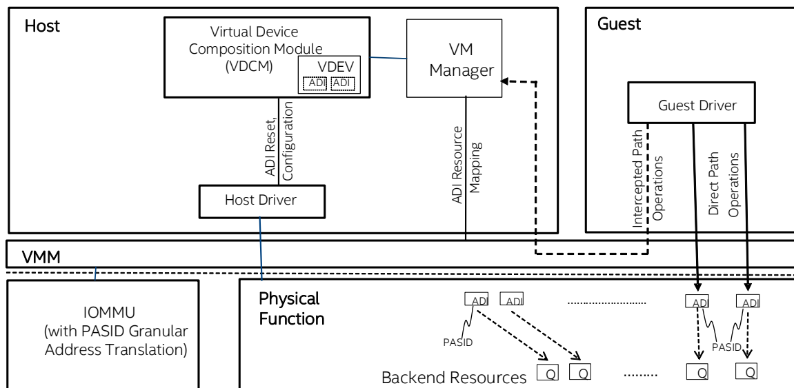
Figure 6-3: Scalable IOV Software Architecture
