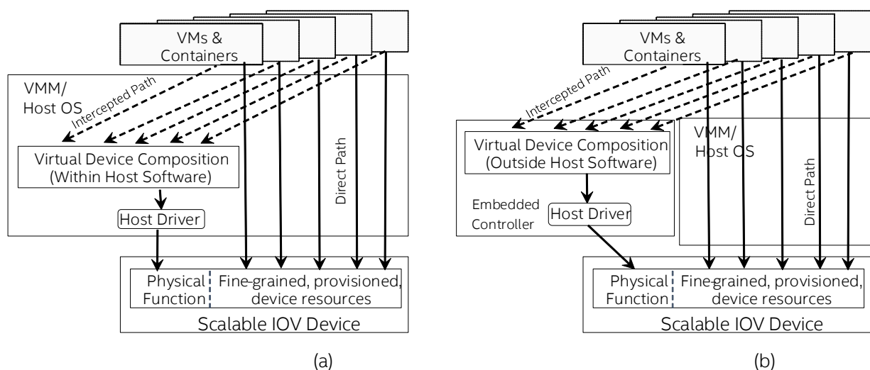
Figure 6-1: Approaches to Scalable IOV
